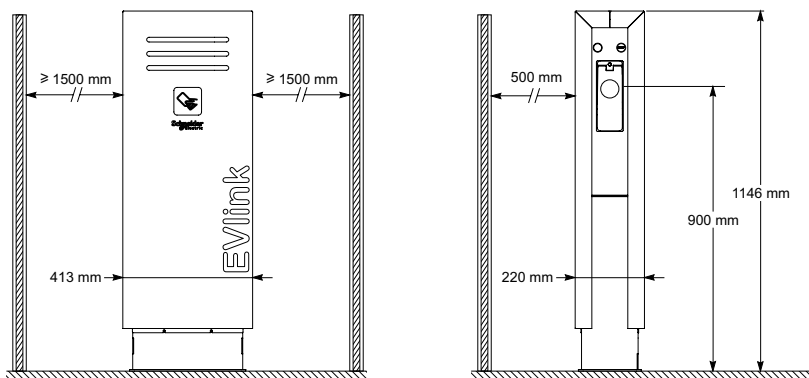
Floor-standing charging station
